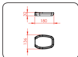
FLAT HAND REST , incl. connecting element with 4 grub screws Part # RPU2
