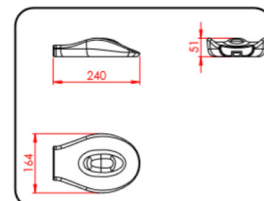
PALM EXTENSOR HAND REST incl. connecting element with 4 grub screws. Fits left or right hand Part # RPUH5
