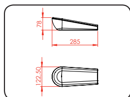
SUPPORT WITH SLOT NUTS for optimal forearm stabilisation and positioning Part # RPU1S
